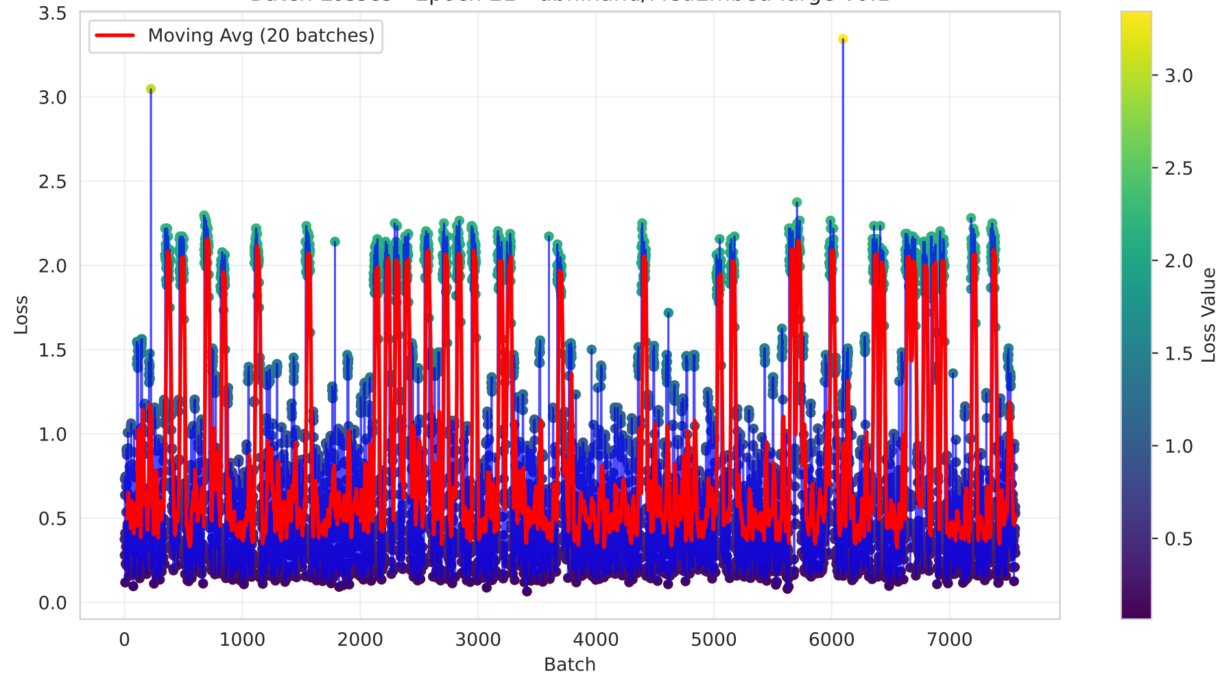
Batch Losses - Epoch 21 - abhinand/MedEmbed-large-v0.1
