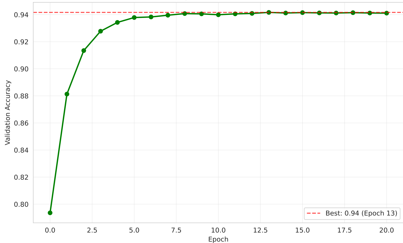
Validation Accuracy - abhinand/MedEmbed-large-v0.1
