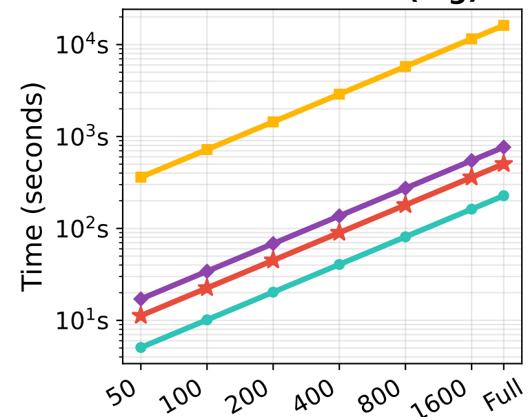
Inference Time (log)
