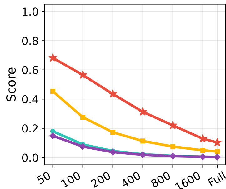
AP
