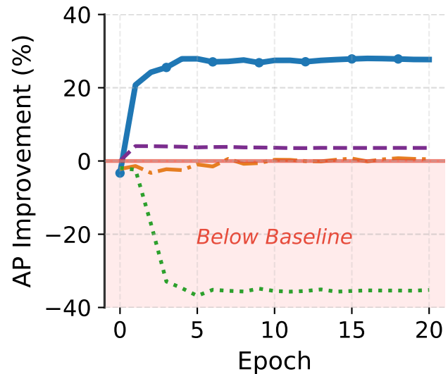
Row-Sentence Alignment
