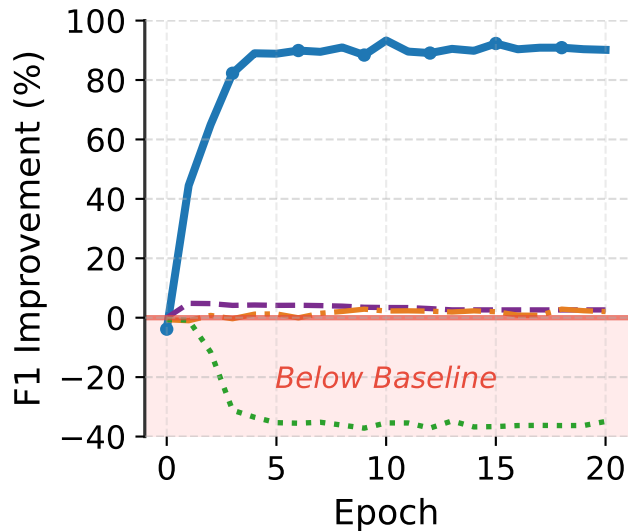
Row-Sentence Alignment
