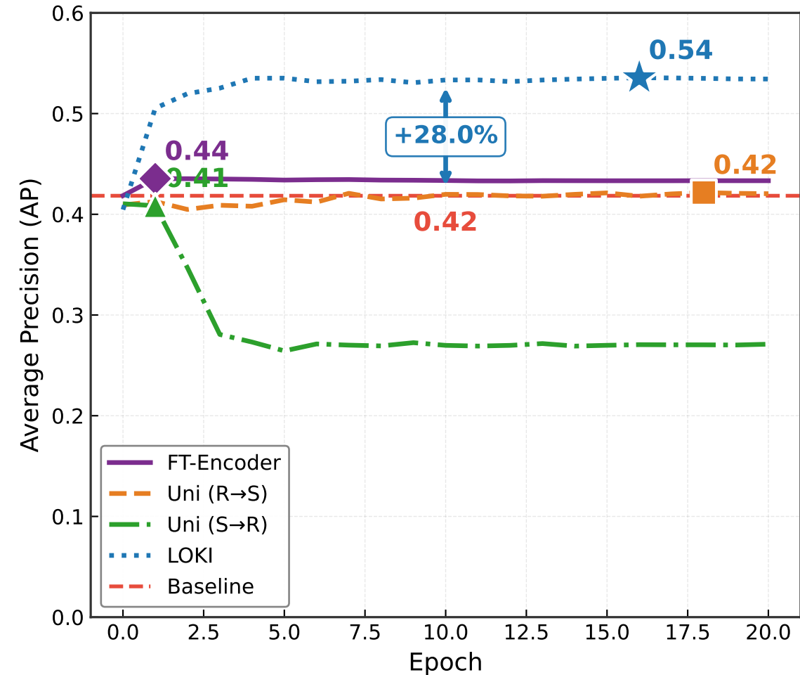
Row-Sentence Alignment: Average Precision (AP)
