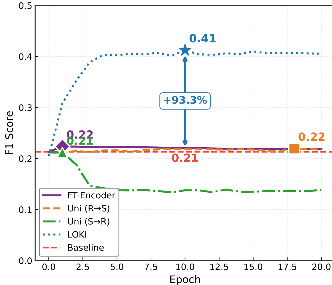
Row-Sentence Alignment: F1 Score
