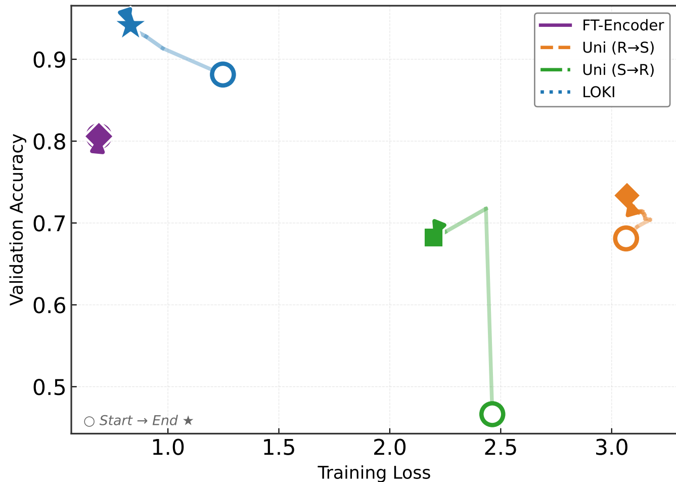
Training Trajectory: Loss \rightarrow Accuracy
