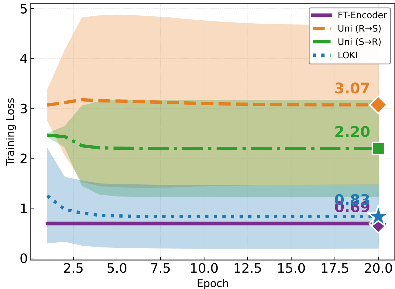
Training Loss (Mean \pm Std)
