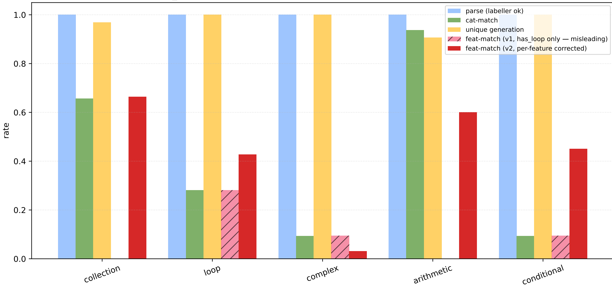
python_code reverse-bridge scorecard — v2 validator corrects v1 feat-match
