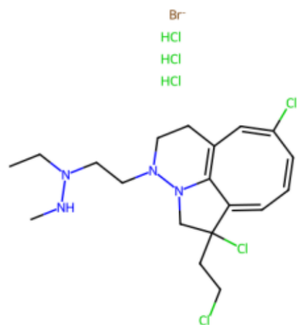
complex-polycyclic p1565 MW 607
