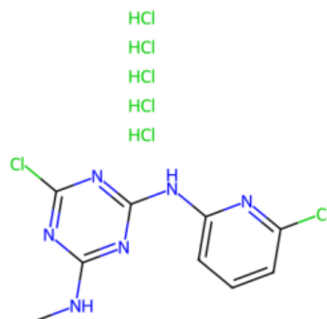
functional-rich p1562 MW 307
