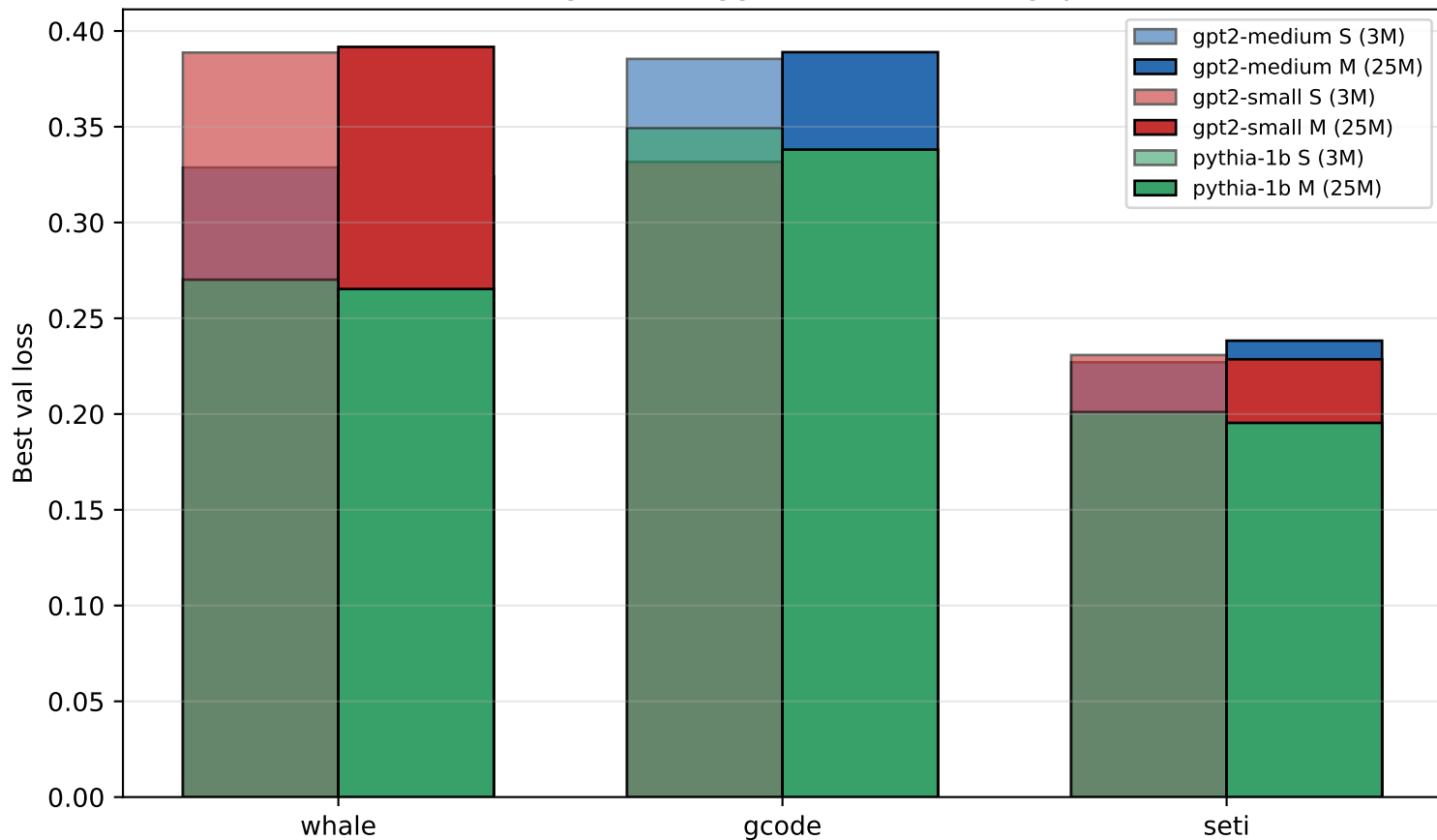
S-model scaling: does bigger S close the SS gap at scale?
