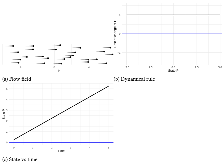
Figure 13.6.: Flow field when dynamical rule is \text{flat}() .
