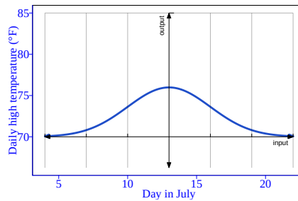
Figure 7.6.: hill( )
