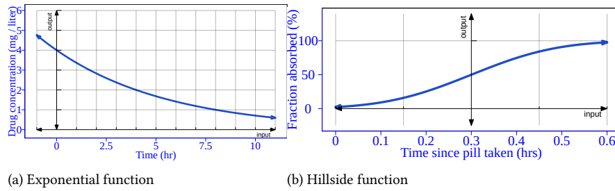
Figure 9.1.: These core modeling functions cover different aspects of the drug absorption and elimination processes.
