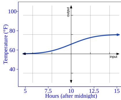
Figure 7.5.: hillside( )
