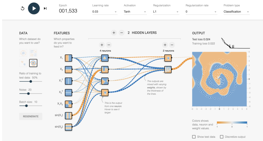
Figure 16.7.: A snapshot from a demonstrator web app showing training for a simple neural network model. You can interact with the demonstrator at https://playground.tensorflow.org/
