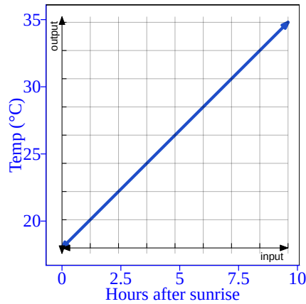
Figure 7.9.: same()
