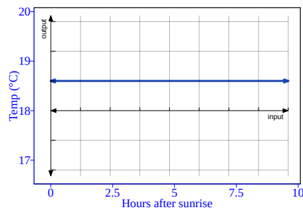
Figure 7.10.: flat()
