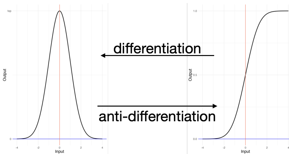
Figure 15.3: hill() and hillside() are a derivative/anti-derivative pair.
