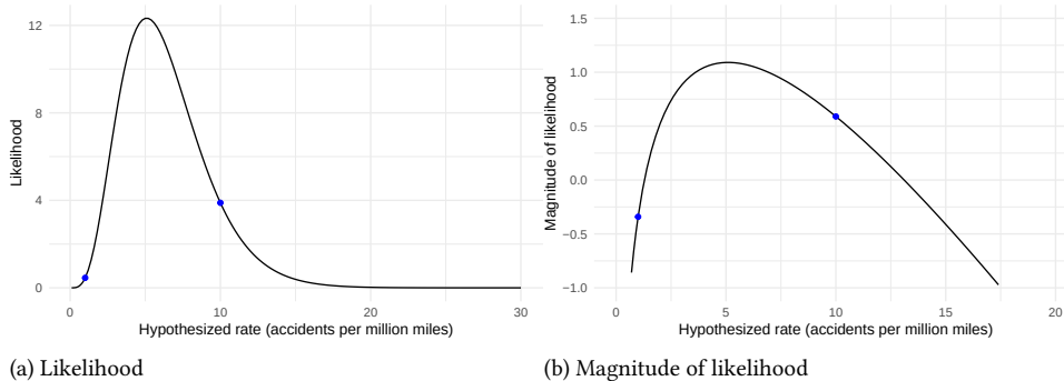
Figure 12.3.: Likelihood (with respect to the data in r_xf('tbl-car-crash-table') ) as a function of the hypothesized accident rate. The blue dots indicate the two advocates' hypotheses.
