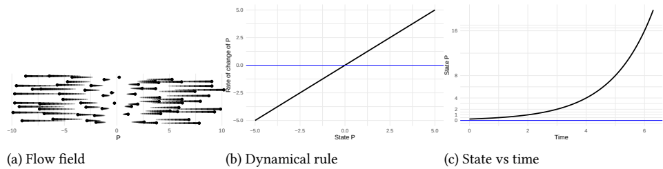
Figure 13.7.: Flow field when dynamical rule is same() .
