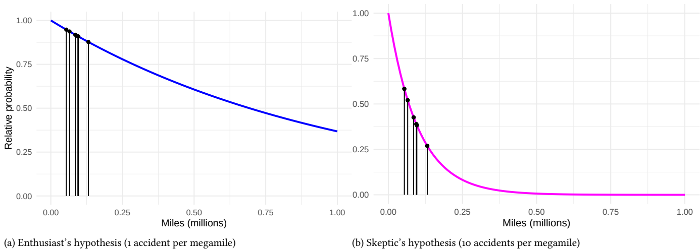
Figure 12.2.: Probability distributions for the mileage without an accident.
