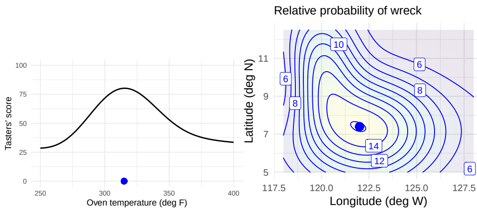
Figure 10.1: The argmax (blue dot) for each of two example objective functions.
