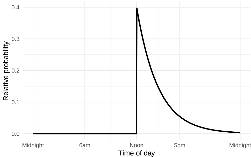
Figure 8.4.: The exponential distribution.
