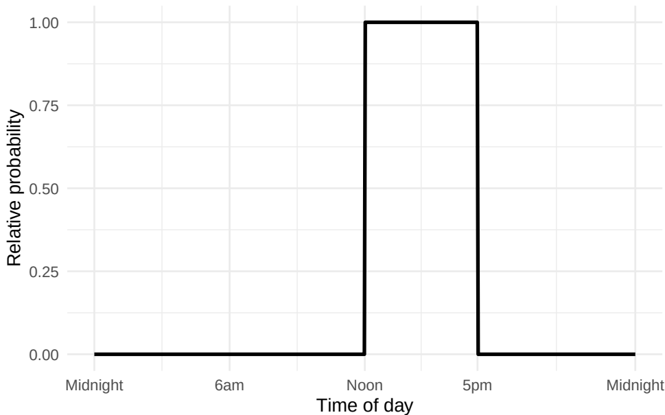
Figure 8.2.: A uniform distribution.
