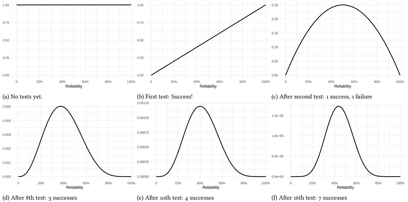
Figure 12.5.: The initial prior for the success rate and posteriors calculated at several points in the string of 16 tests (which had 7 successes).
