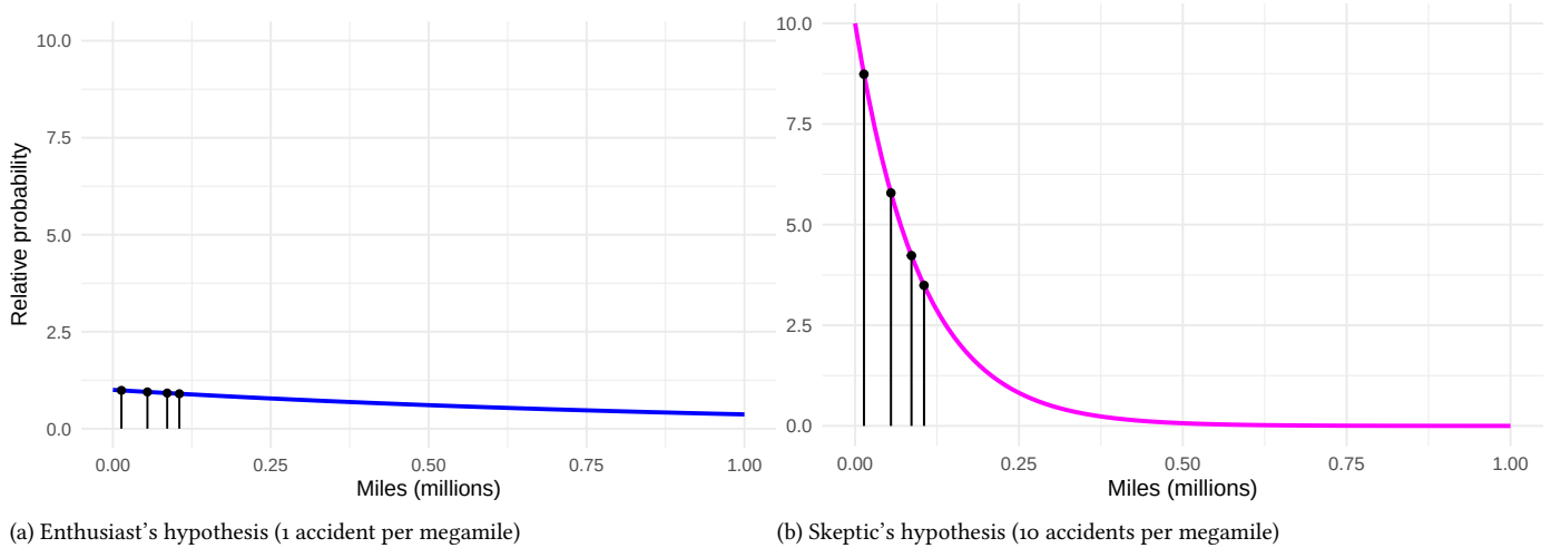
Figure 12.1.: Probability distributions for the mileage until an accident, according to the skeptic's and enthusiast's competing hypotheses. The length of the black line gives the probability for each event, according to the hypothesis.
