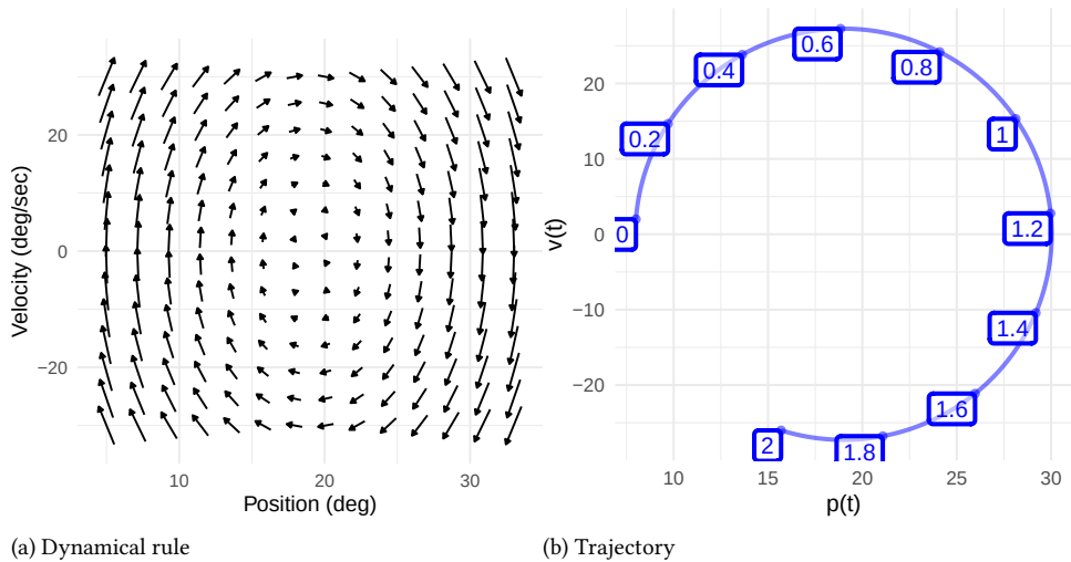
Figure 13.2.: The dynamical rule for the system of r('fig-pendulum-gif') . The rate of change at selected points in the state space is a vector since both components of the state are changing.
