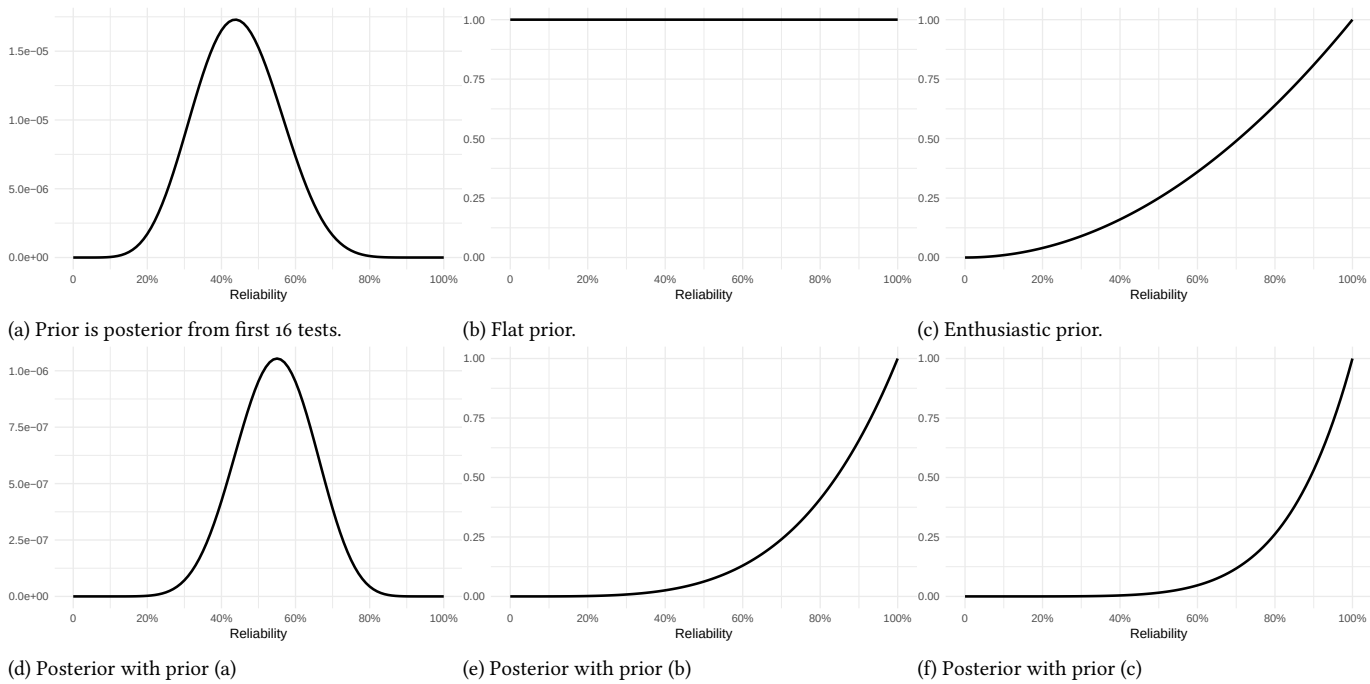
Figure 12.6.: Posteriors after the last 4 ICBM successful interceptor tests. Three different priors are considered.
