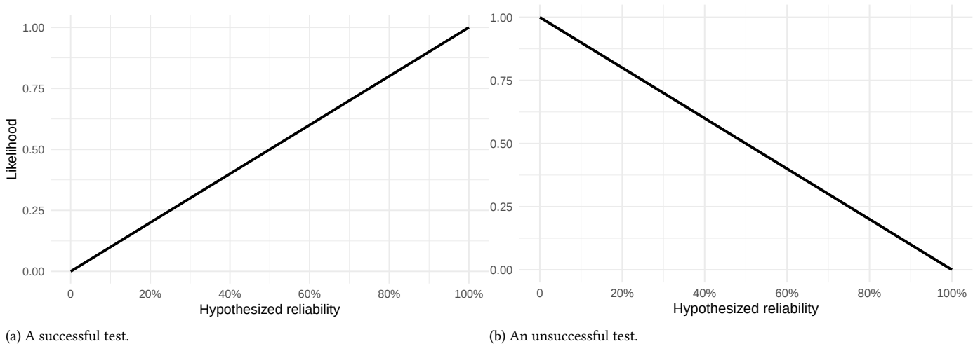
Figure 12.4.: Likelihood functions for the outcome of a yes/no test.
