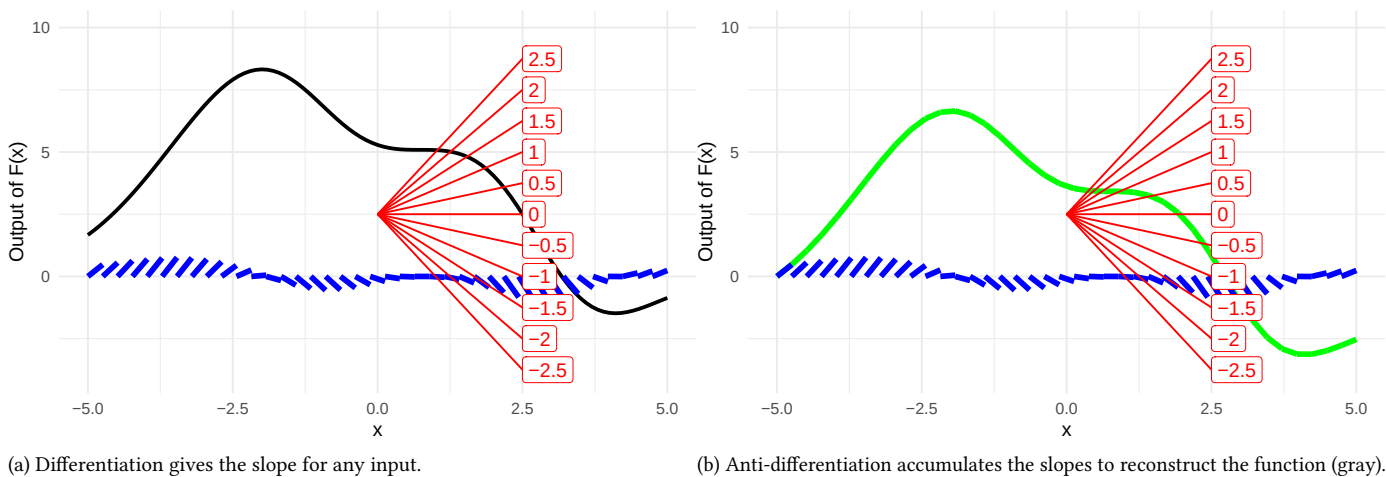
Figure 15.4.: A function (black) with its rate-of-change function depicted as short inclined segments (blue).
