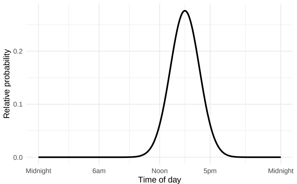
Figure 8.3.: A normal distribution smooths out the sharp corners of Figure 8.2.
