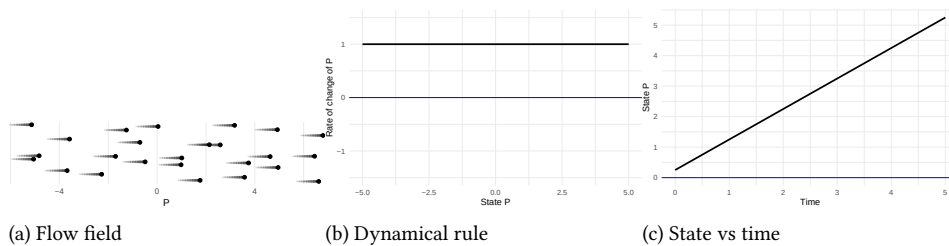
Figure 13.6.: Flow field when dynamical rule is flat() .
