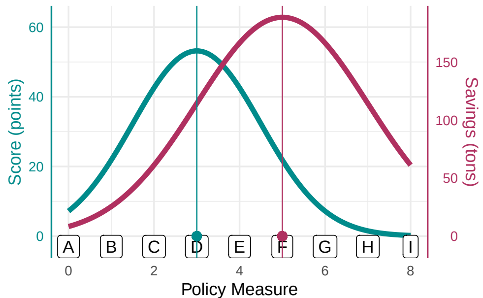
Figure 10.3: Two objective functions whose outputs have different dimension.
