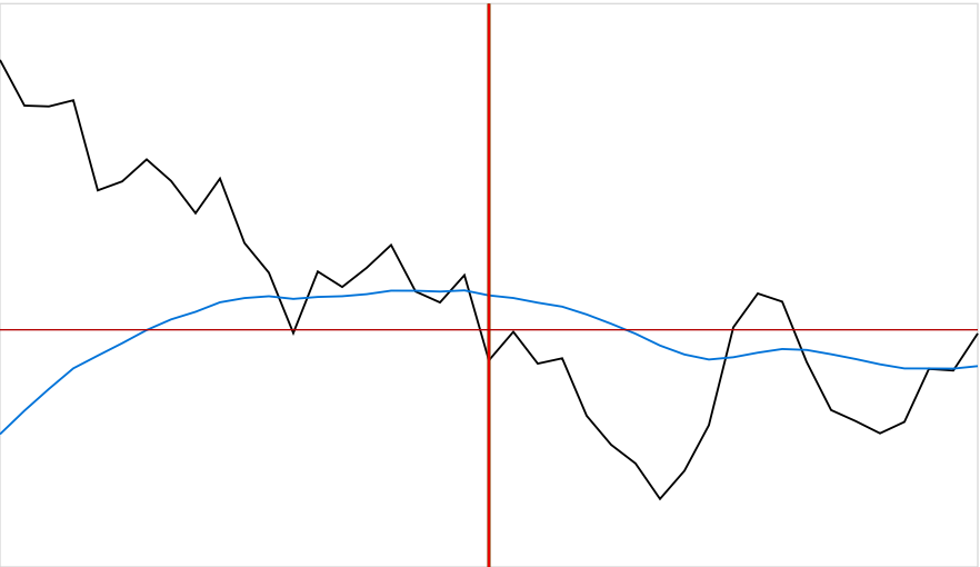
ENTRY_A_STOP_A_EXIT_A_TRAIN_0018
