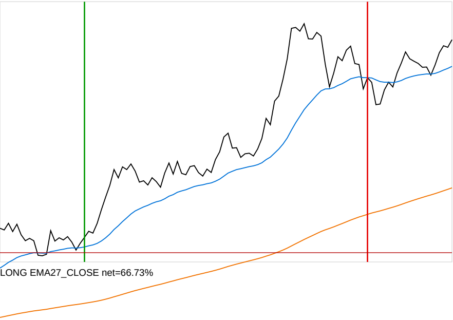
ENTRY_A_STOP_B_EXIT_B_TRAIN_0036
