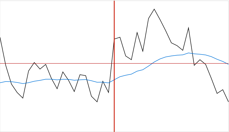
ENTRY_A_STOP_A_EXIT_A_TRAIN_0008
