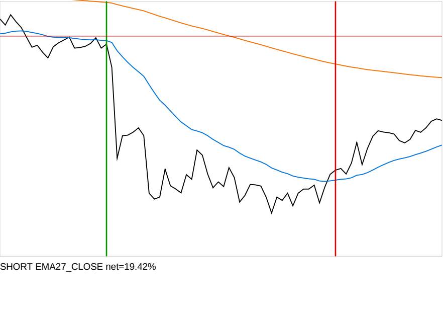
ENTRY_A_STOP_A_EXIT_A_TRAIN_0032
