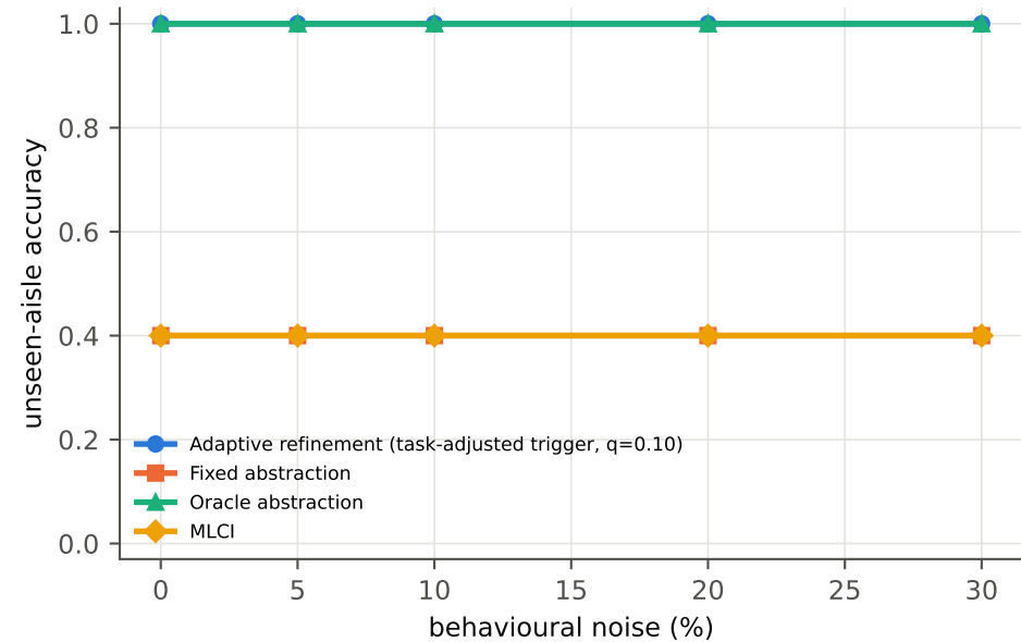
Exp. 2 unseen aisle - behavioural noise
