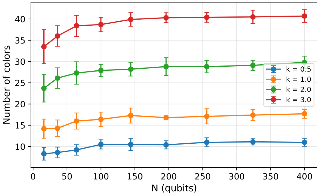
Parent-Level Graph Coloring
