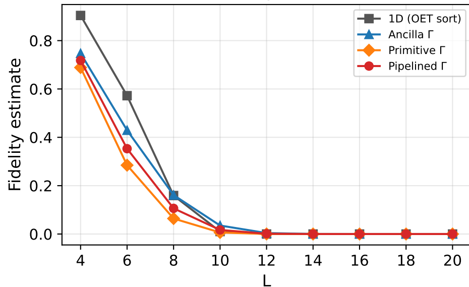
Reversal, p = 1e-03
