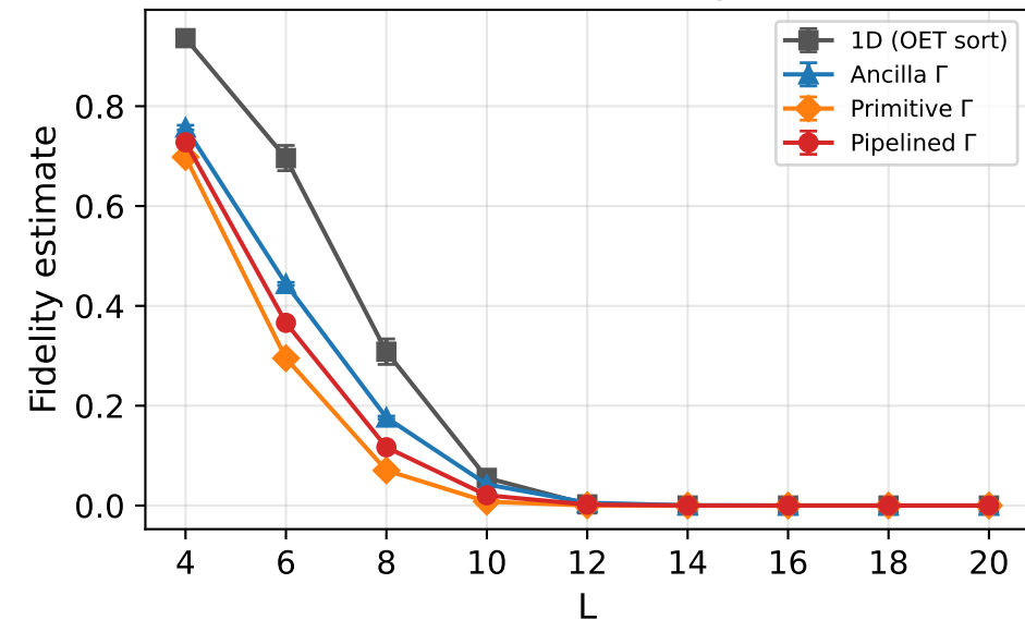
Random (mean \pm std), p = 1e-03
