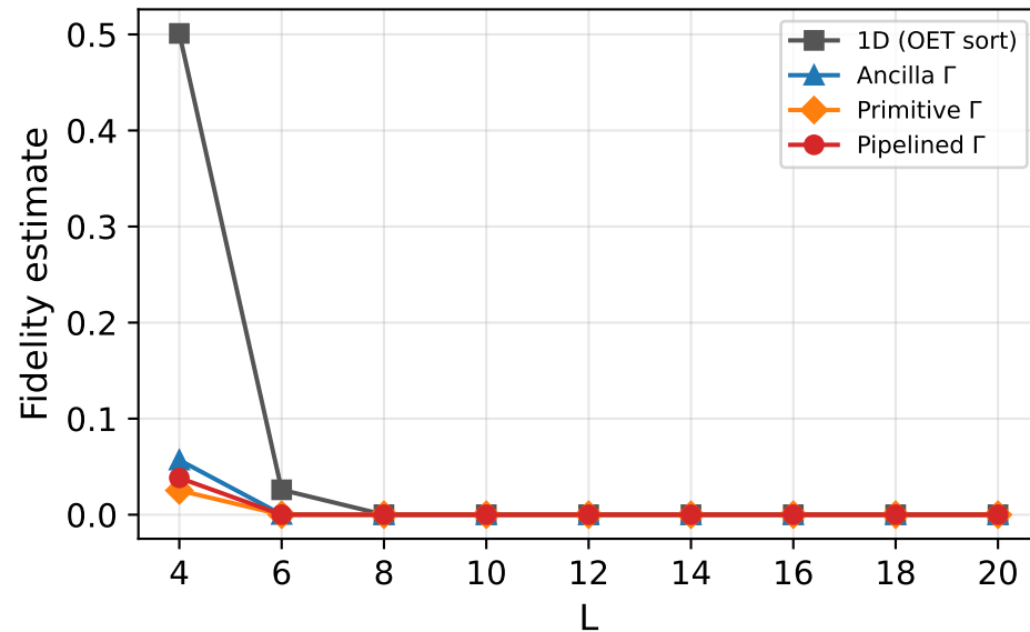
2D Reflection, p = 1e-02
