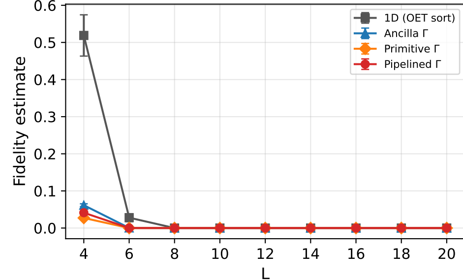
Random (mean \pm std), p = 1e-02
