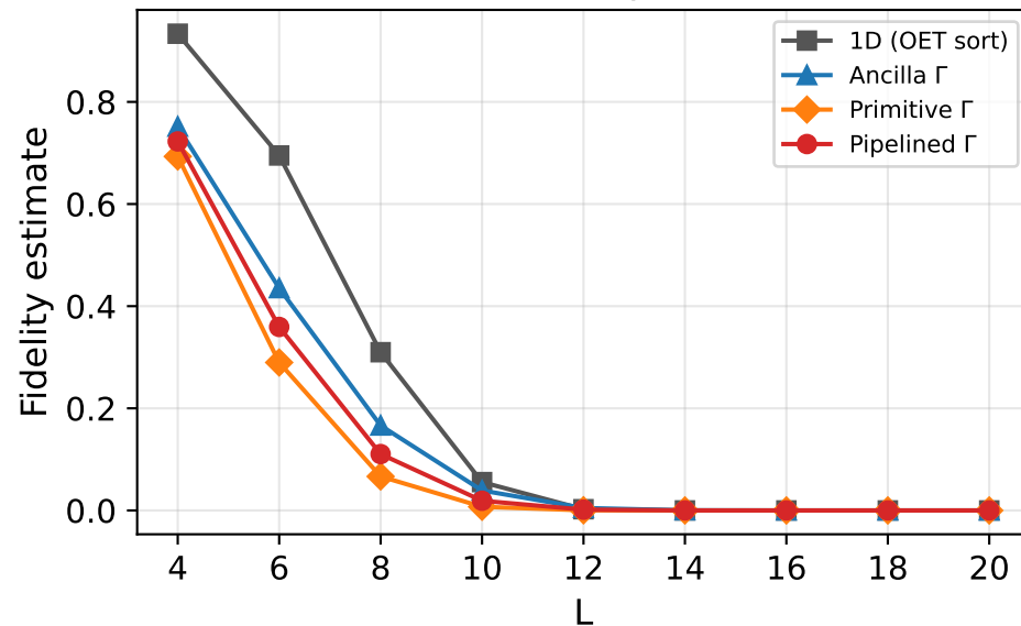
2D Reflection, p = 1e-03
