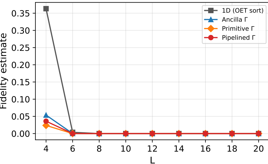
Reversal, p = 1e-02
