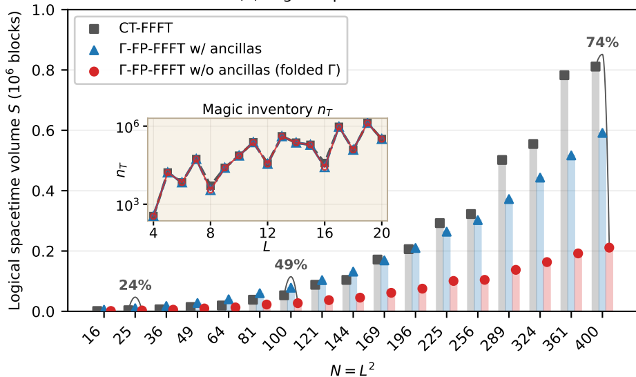
(a) Logical spacetime volume
