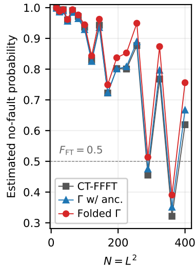
(b) Estimated no-fault probability ( d = 11 )
