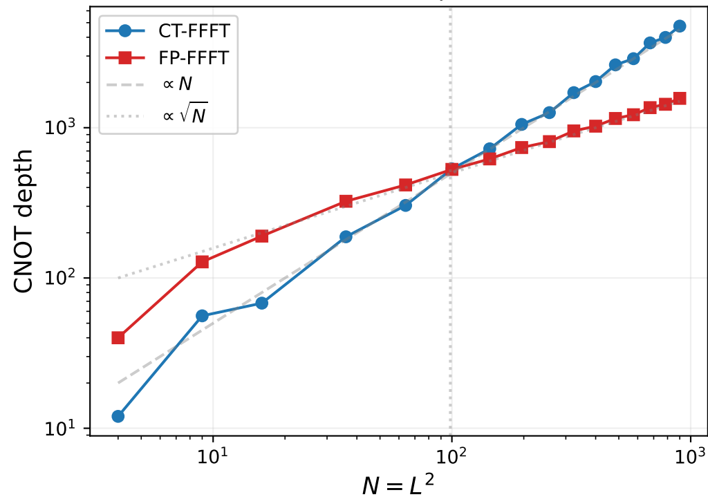
Circuit Depth
