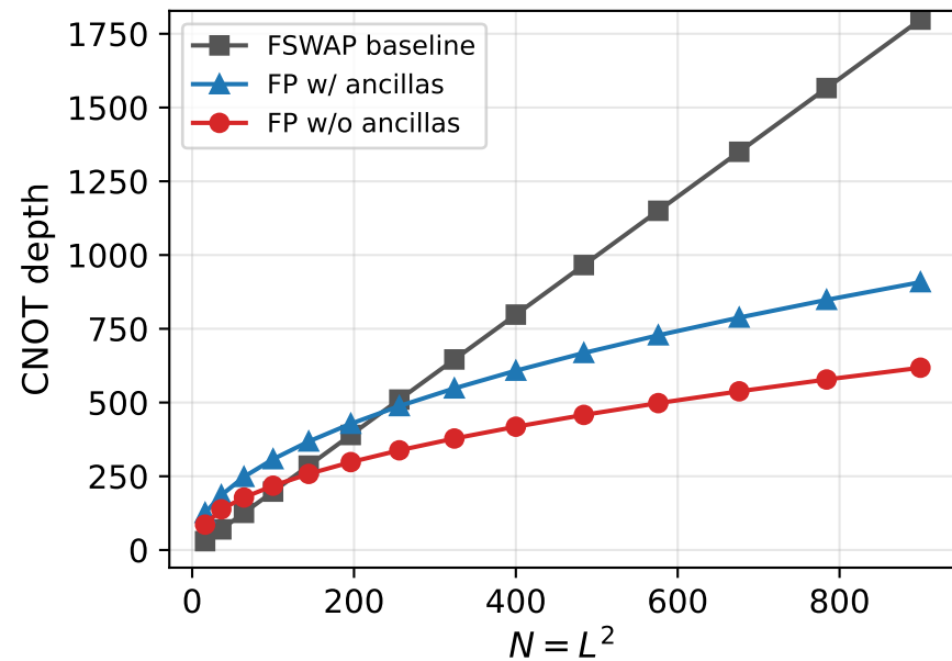
Reversal
