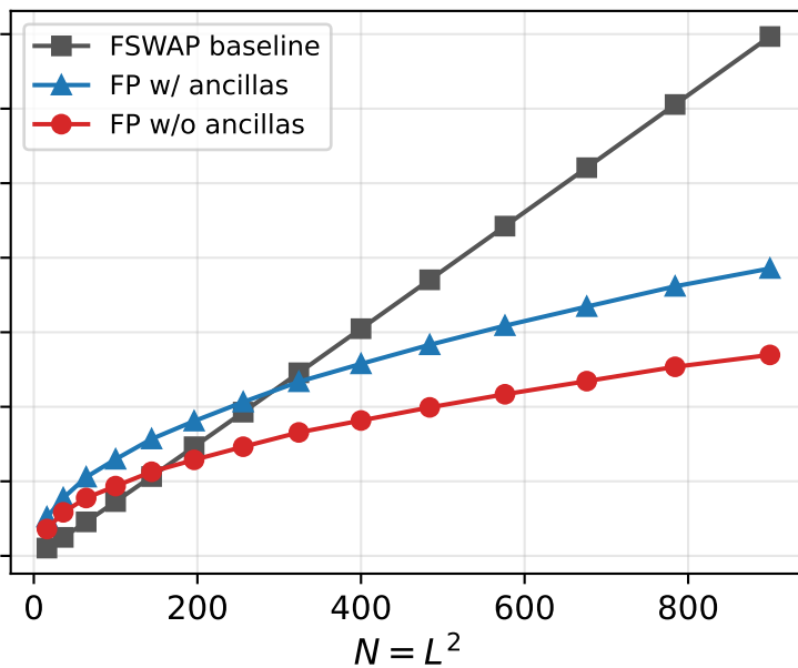
2D Reflection
