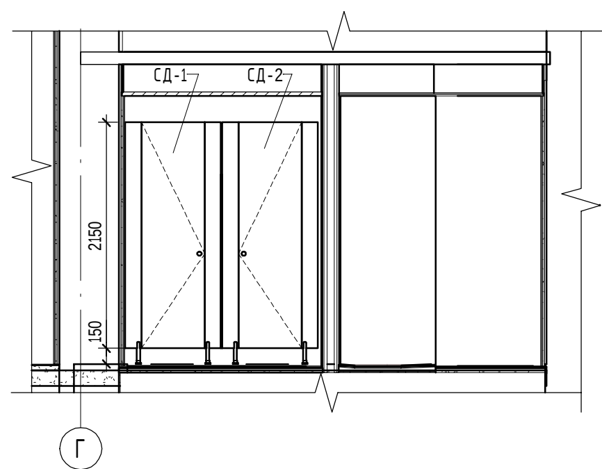
4-4
