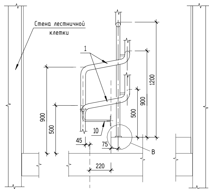
2-2
