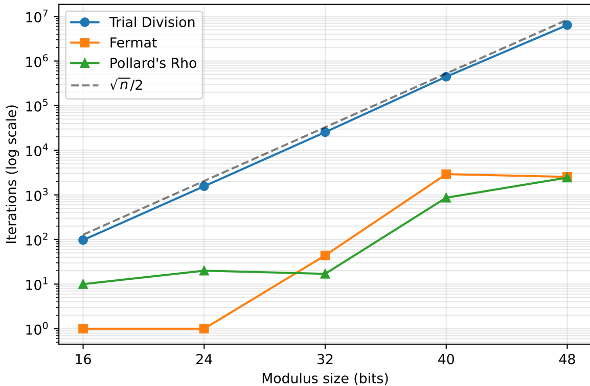
Iterations needed to factor n
