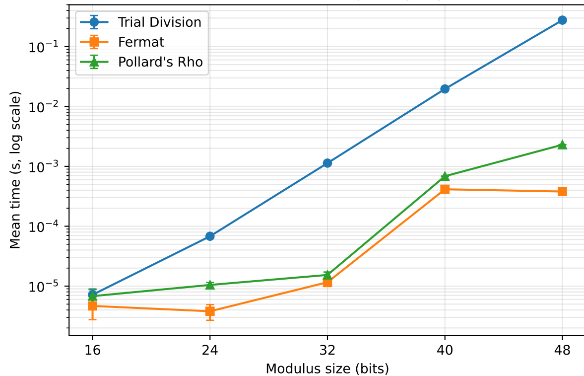
Factorization time (3 repeats per point)
