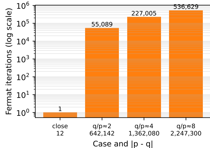
Fermat factorization vs |p - q| (40-bit moduli)
