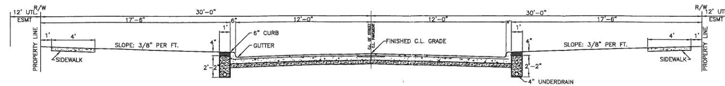
TYPICAL PAVEMENT SECTION NO SCALE
