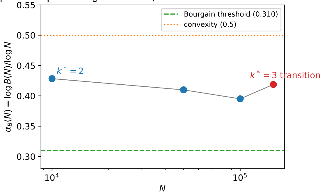
Empirical exponent \alpha_B : decrease, then reversal at the k = 3 transition
