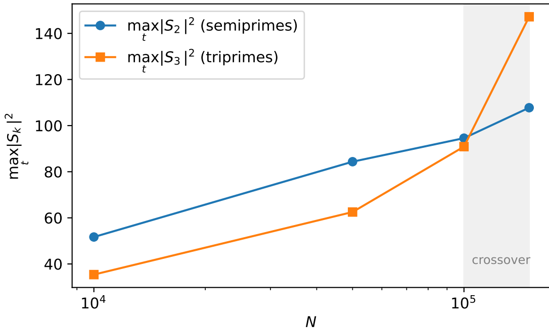
The k = 2 \rightarrow k = 3 dominance transition near N \approx 10^5
