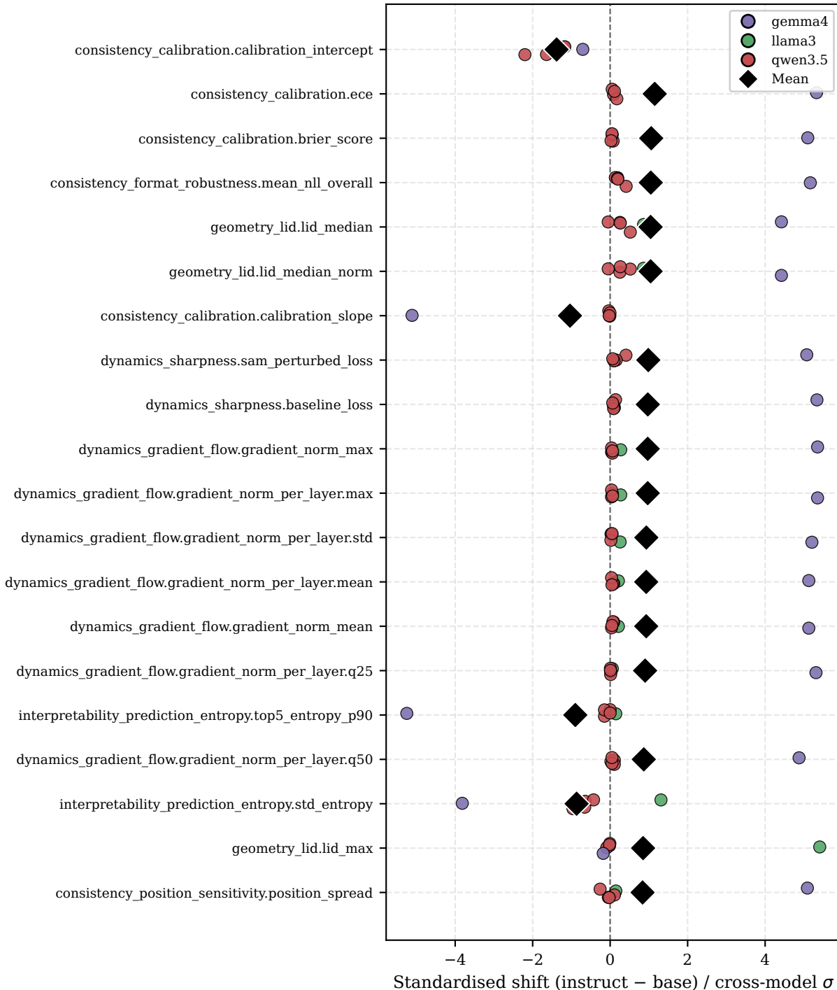
Largest 20 intrinsic-property shifts after instruction tuning (per-pair markers; black \diamond = mean over n = 6 pairs)
