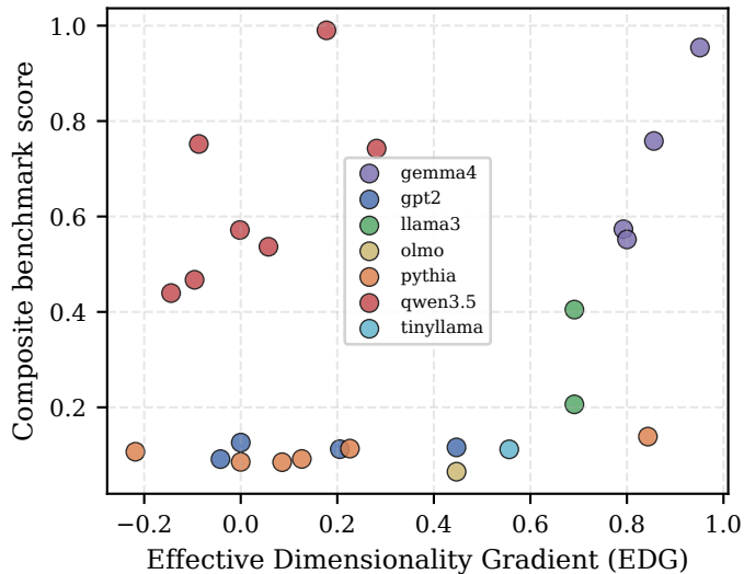
(a) EDG predicts capability ( \rho = 0.26 , p = 2.1e - 01 )
