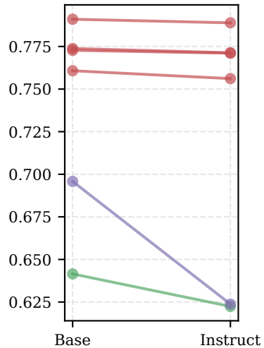
MLP sparsity L_0
