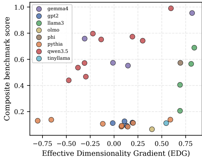
(a) EDG predicts capability ( \rho = 0.11 , p = 5.4e-01 )
