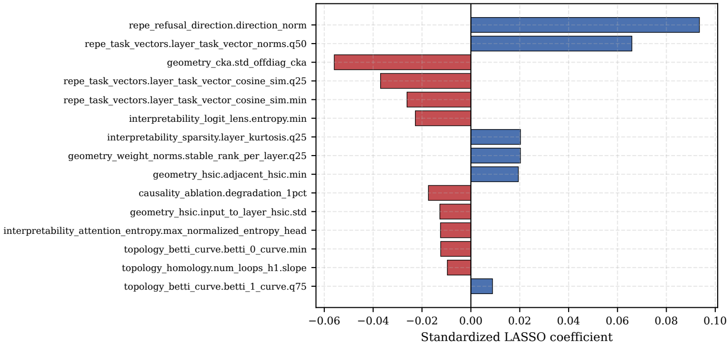
Top 15 features predicting composite benchmark score
