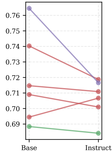
Refusal direction AUROC
