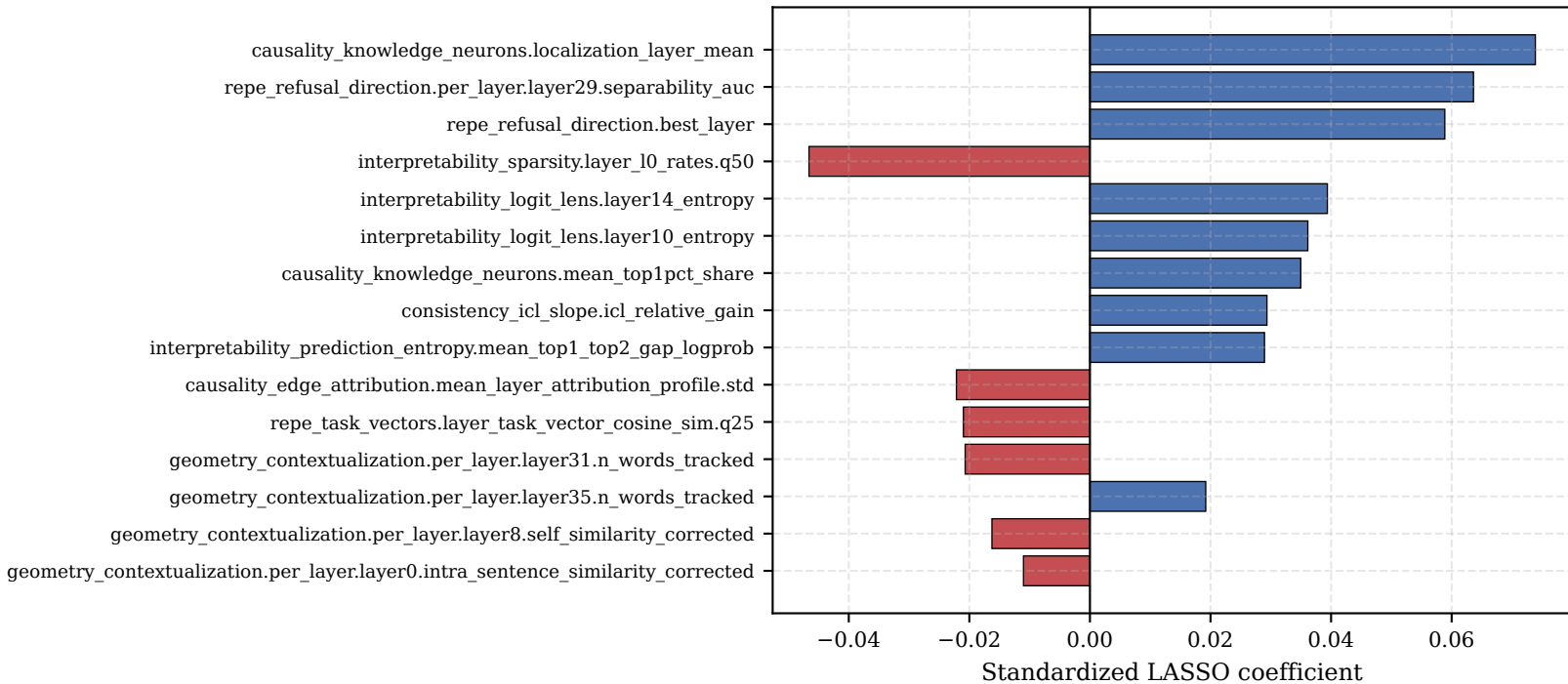
Top 15 features predicting composite benchmark score
