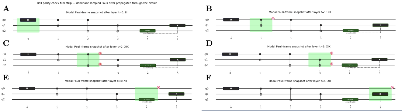
Figure 1: Layer-by-layer Pauli-frame snapshots for a single-shot run on a 3-qubit circuit, exported as a static filmstrip from the CircuitAnimator . At each timestep, the operation time is highlighted with a green box that advances through the circuit left to right, and the current Pauli error operator is carried as a floating label just above the affected qubit wire. (A) Initial circuit layer: no active errors; all qubit wires are in the identity frame. (B) X error injected on the data qubit; the Pauli label appears on the affected wire. (C–D) The X error propagates forward through subsequent entangling gates, spreading to ancilla qubits as the Clifford conjugation rules transform the Pauli frame. (E) Mid-circuit syndrome measurement fires; the classical outcome signals the presence of the error, and the conditional correction is queued. (F) Conditional correction applied; the Pauli frame returns to the identity, confirming successful error detection and correction.
