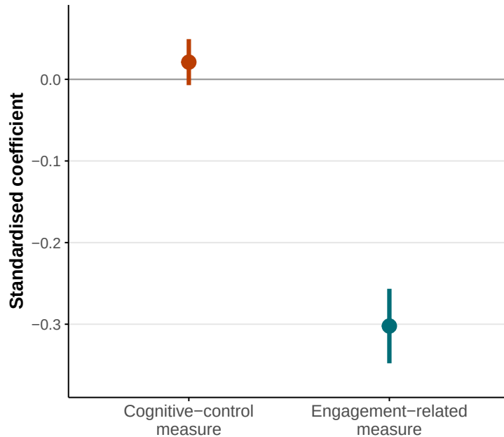
(a) MCS
