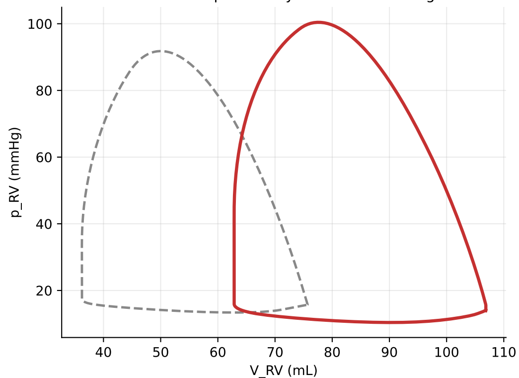
severe RV: peak RV systolic = 100 mmHg
