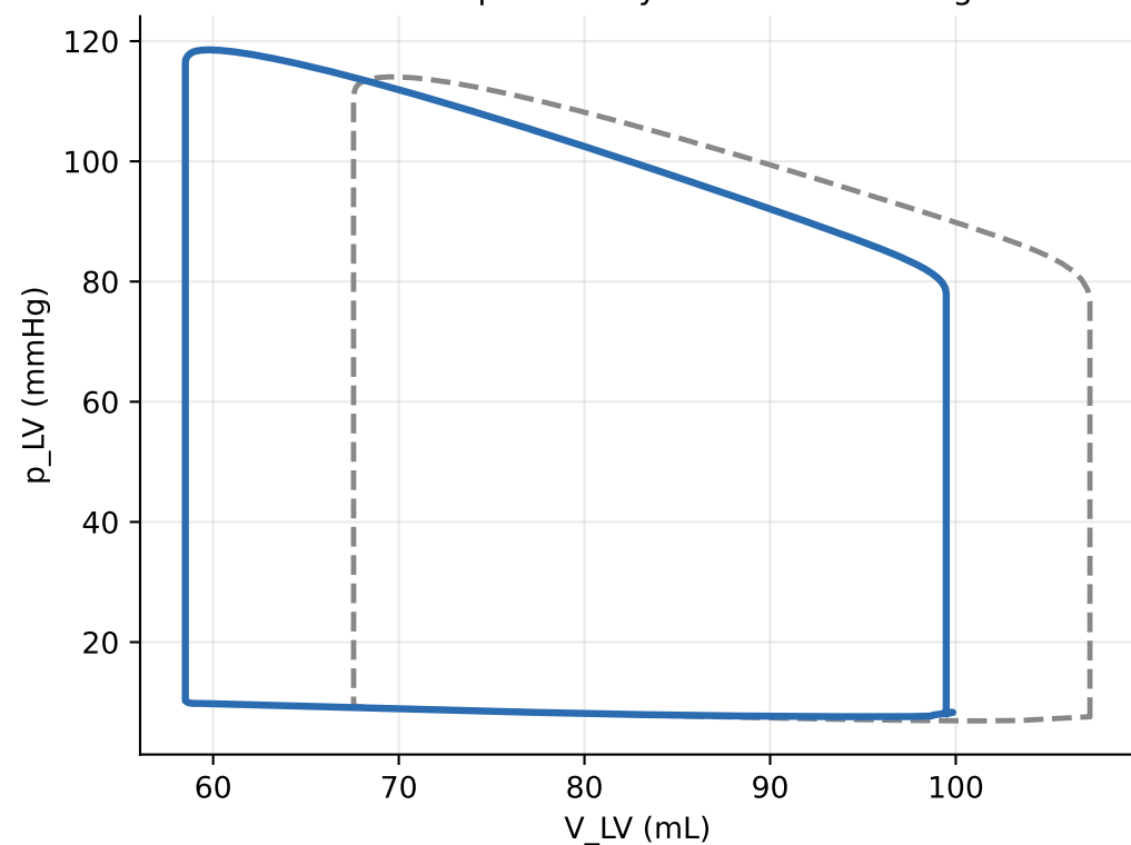
severe LV: peak RV systolic = 100 mmHg
