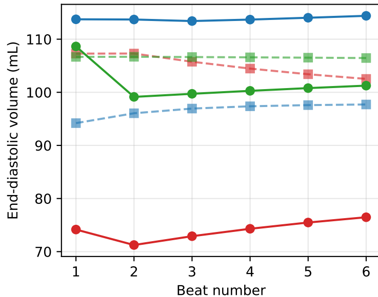
End-diastolic volumes
