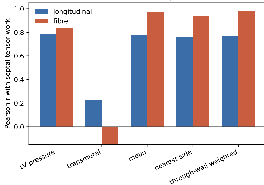
Case ranking
