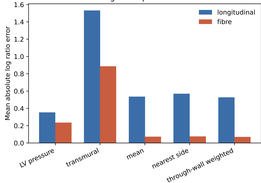
Magnitude preservation
