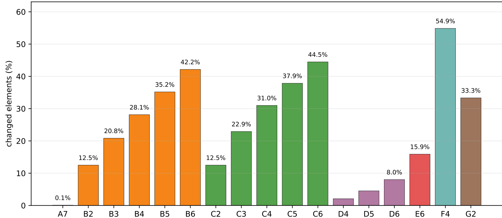
pKL differs from KL in available finite types at p = 2
