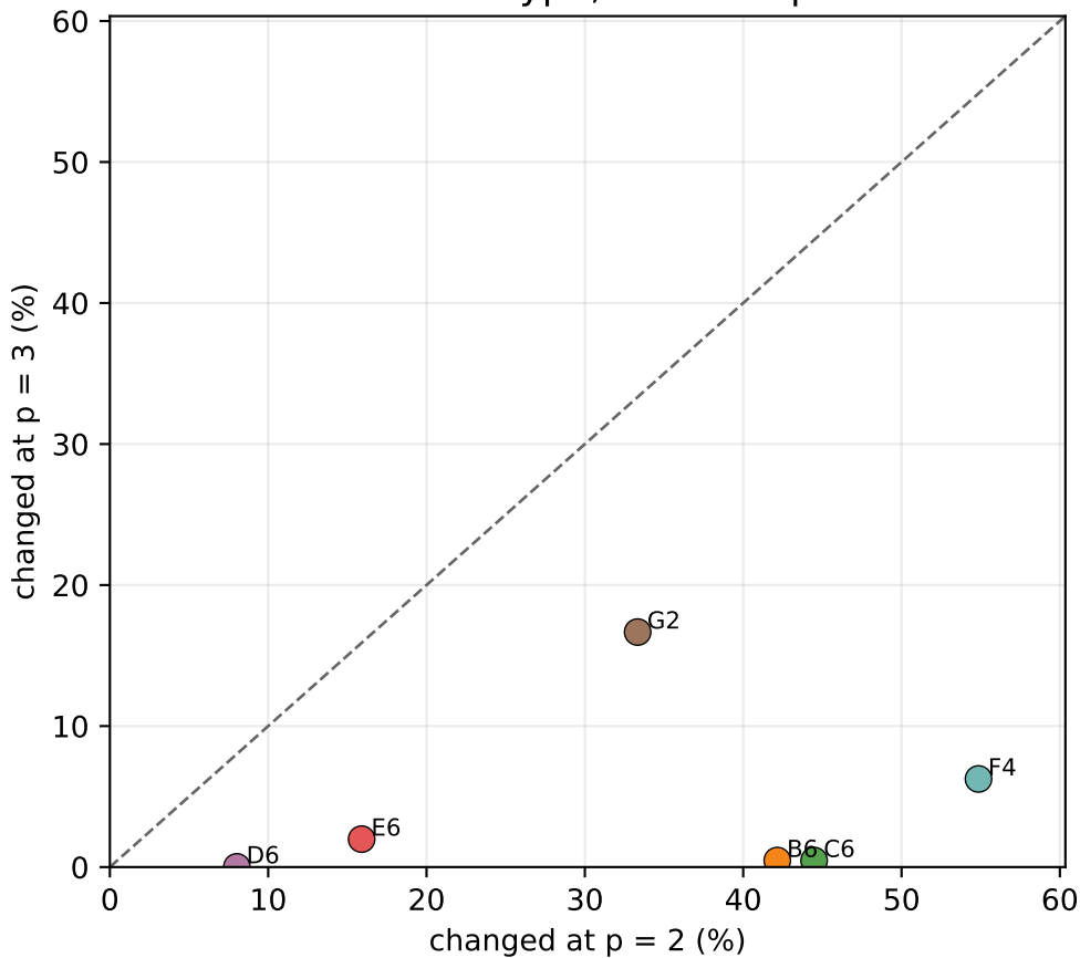
Same finite type, different prime
