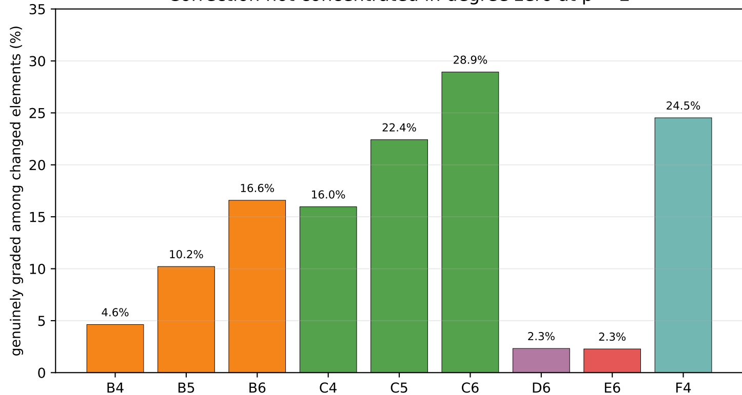
Correction not concentrated in degree zero at p = 2
