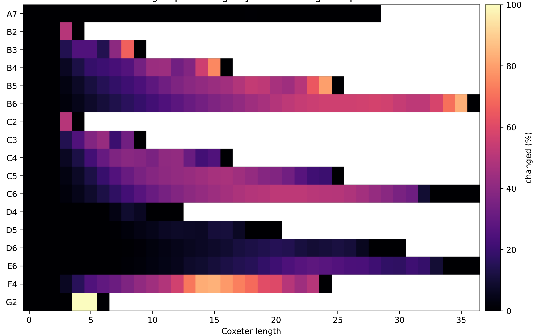
Changed percentage by Coxeter length at p = 2
