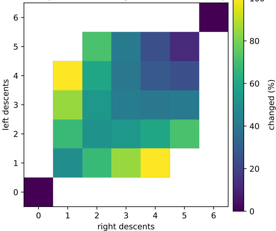
Descent profile of changed elements: C6, p = 2
