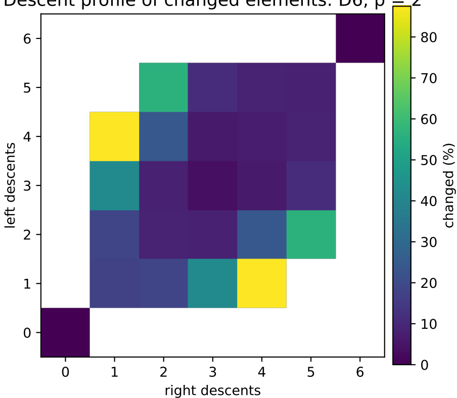
Descent profile of changed elements: D6, p = 2
