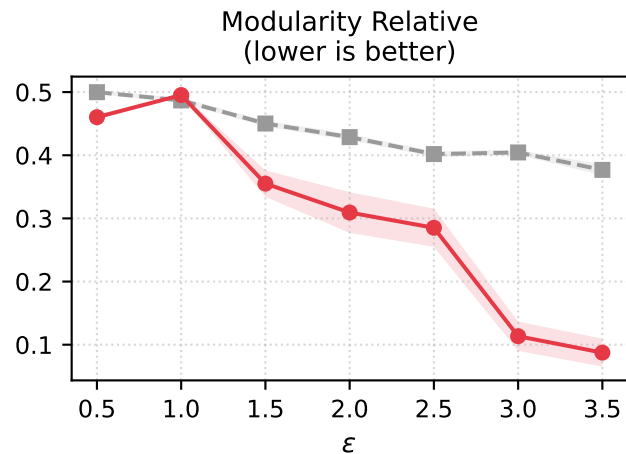
PrivGraph vs Ours on Enron (mean \pm SEM, 10 reps)
