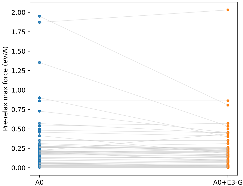
Replication 50000-50063
