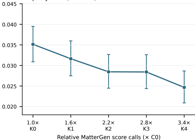
Property MAE (CHGNet)
