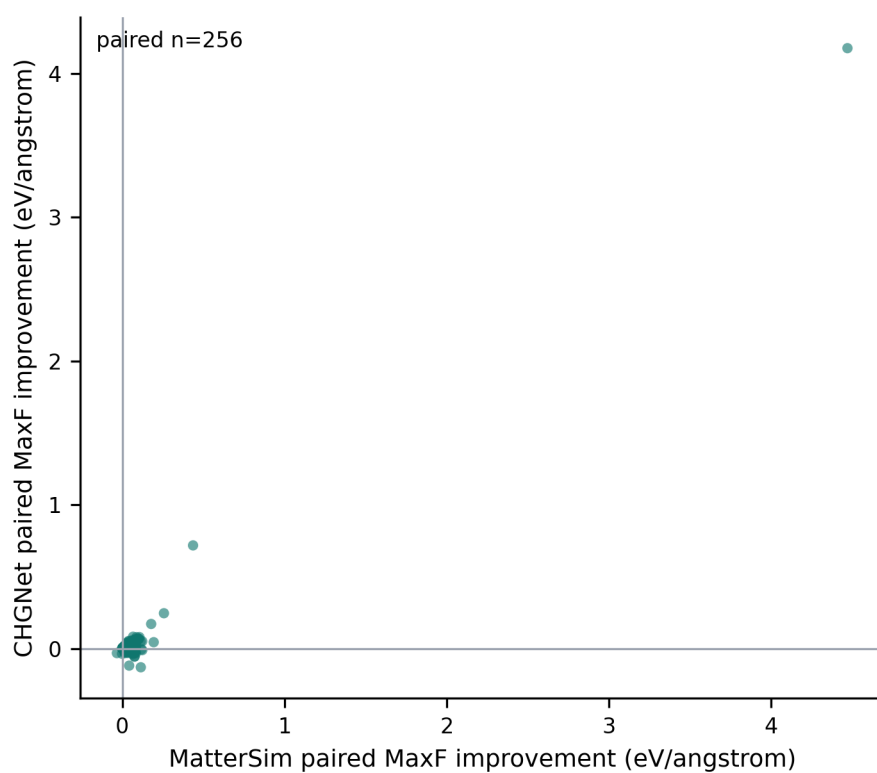
图 5-5: MatterSim 与 CHGNet 的逐样本改善比较 (release ID: I2-F5) Fig. 5-5: Per-Sample Improvement Comparison between MatterSim and CHGNet (release ID: I2-F5)
