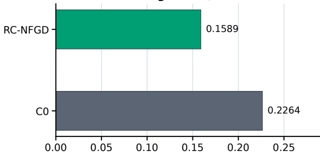
(b) Mean Force [eV/angstrom]; n=256
