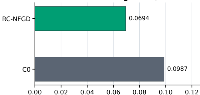
(c) RMSD [angstrom]; n=256
