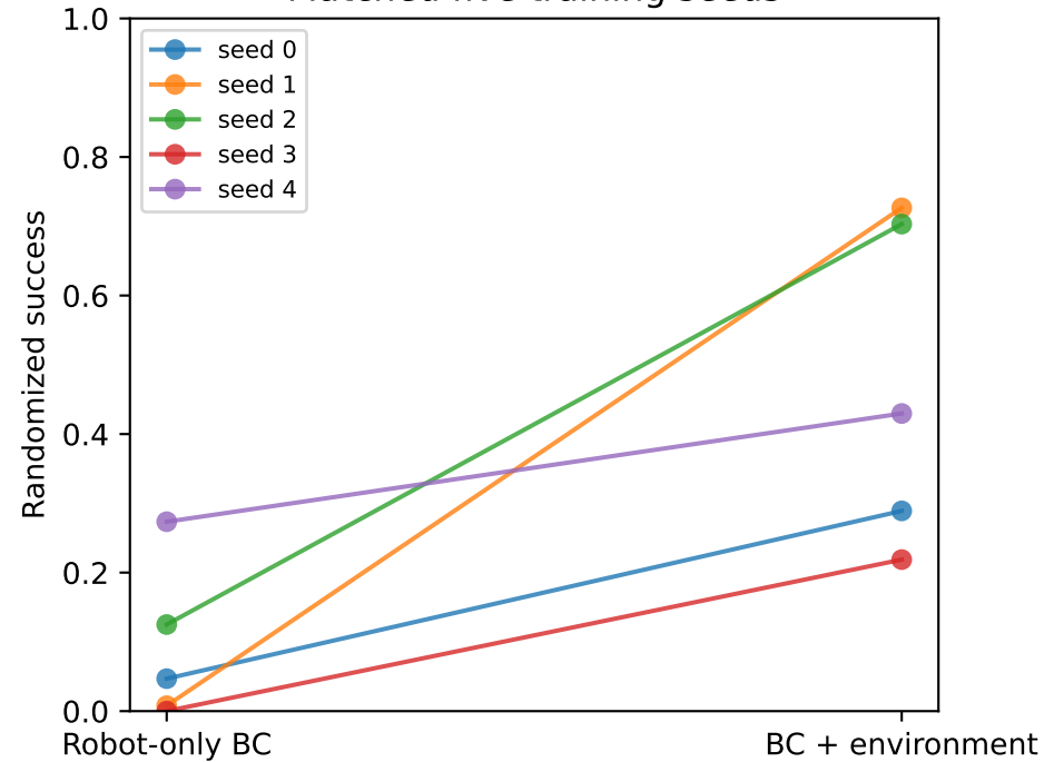
Matched five training seeds
