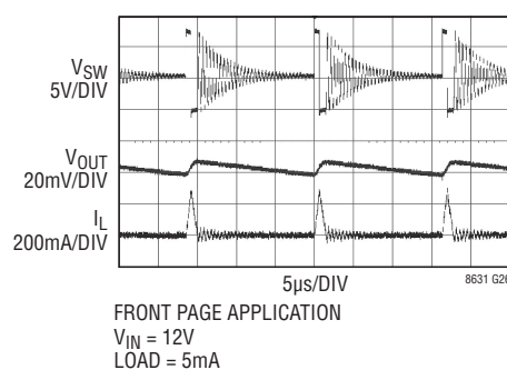
Burst Waveforms
