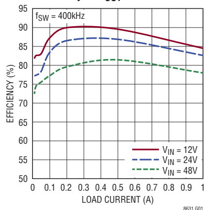
Efficiency at V_{OUT} = 5V
